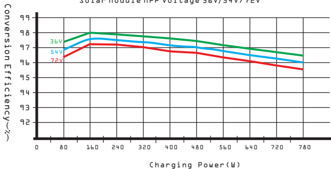
24V Conversion Efficiency Curves Solar Module MPP Voltage 36V/54V/72V
