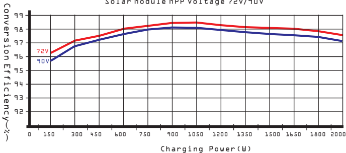
48V Conversion Efficiency Curves Solar Module MPP Voltage 72V/90V
